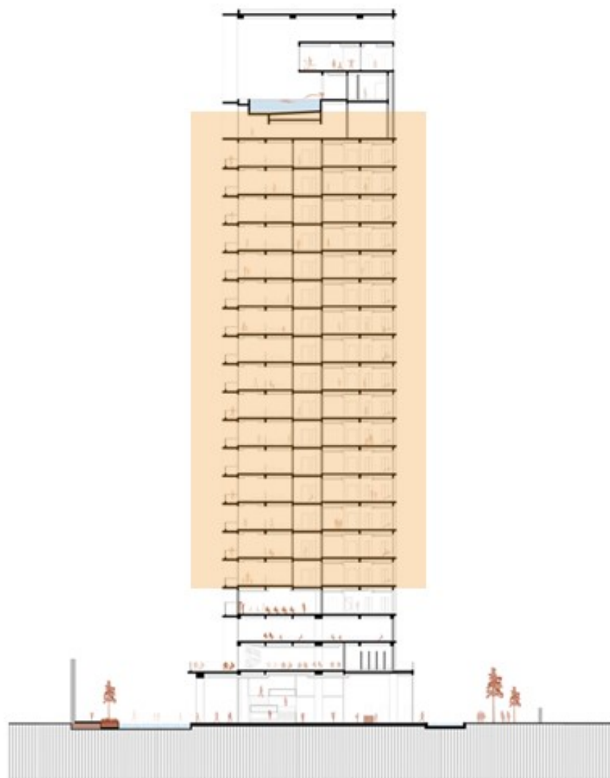
Section D-D'
