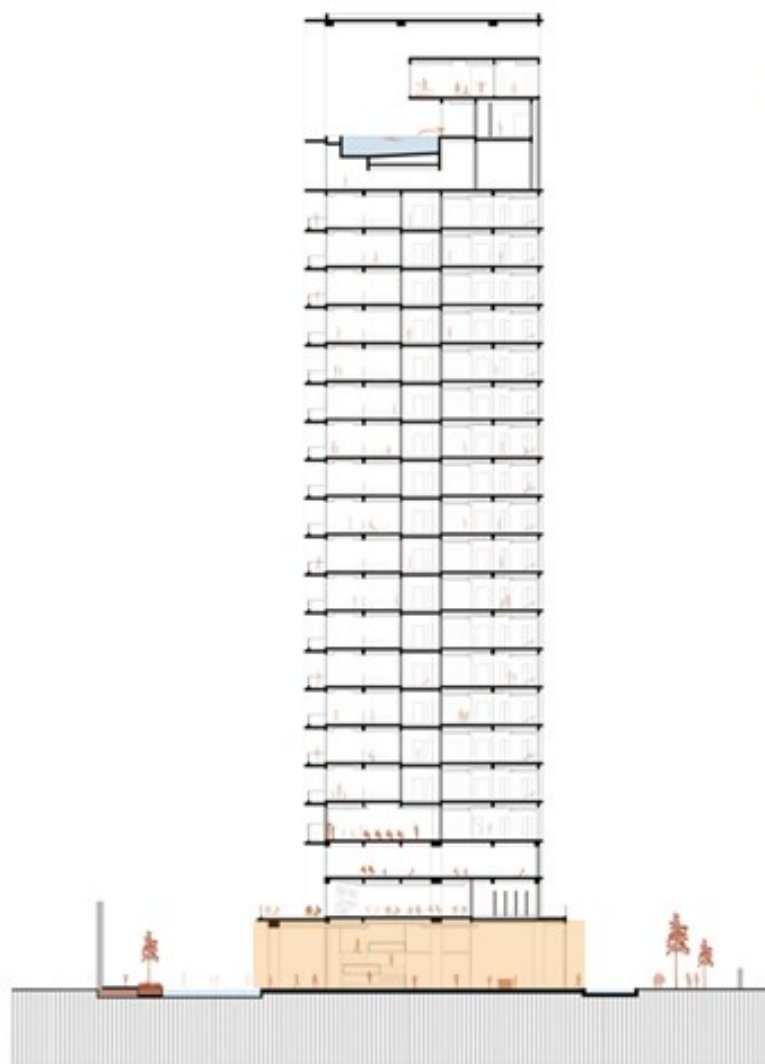
Section D-D' 5 m 10 m 20 m
