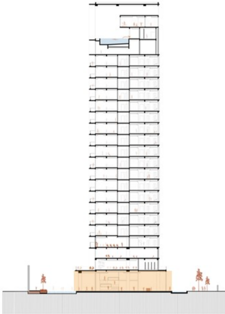
Section D-D'
